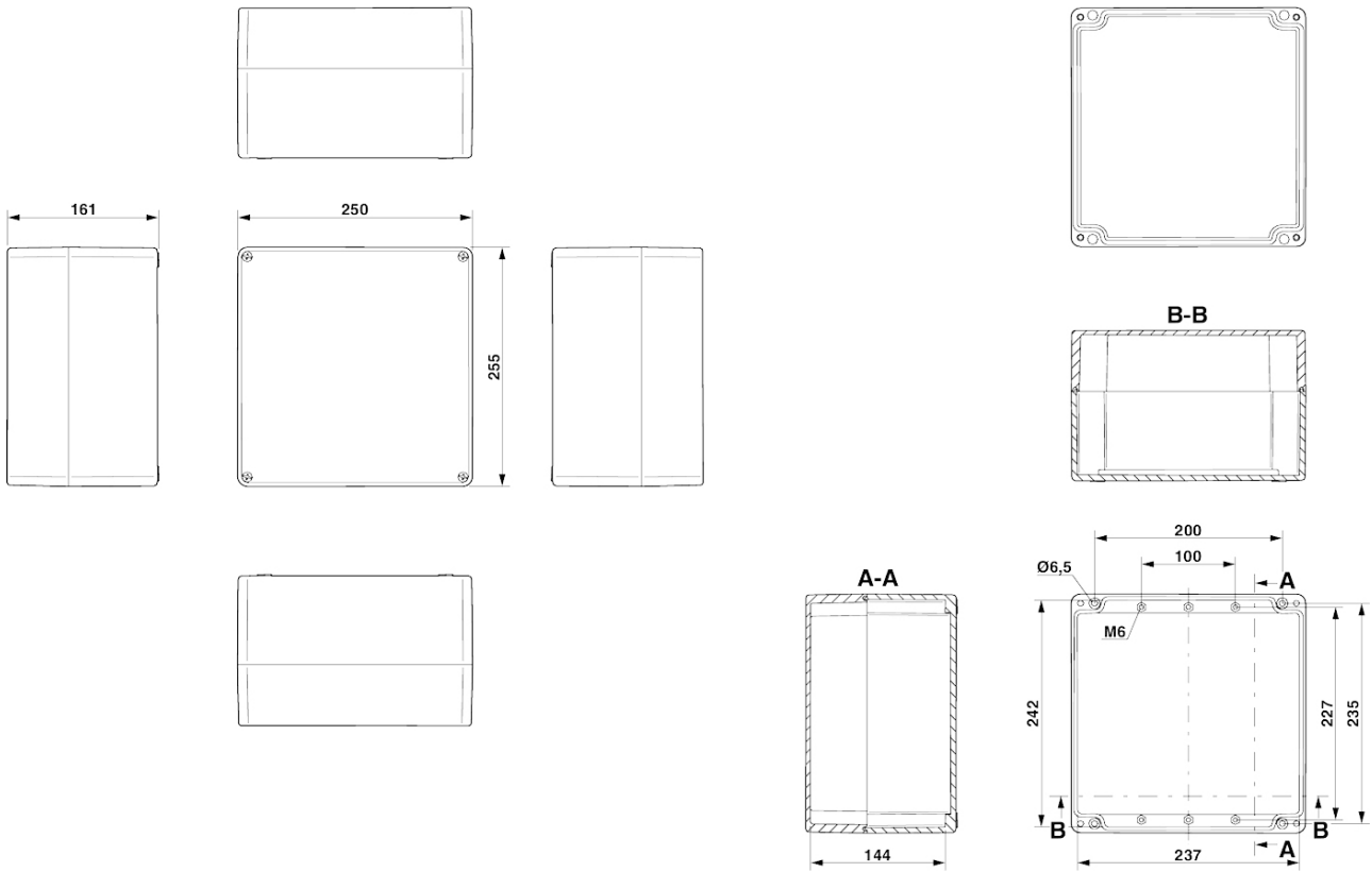
Dimensional drawing
